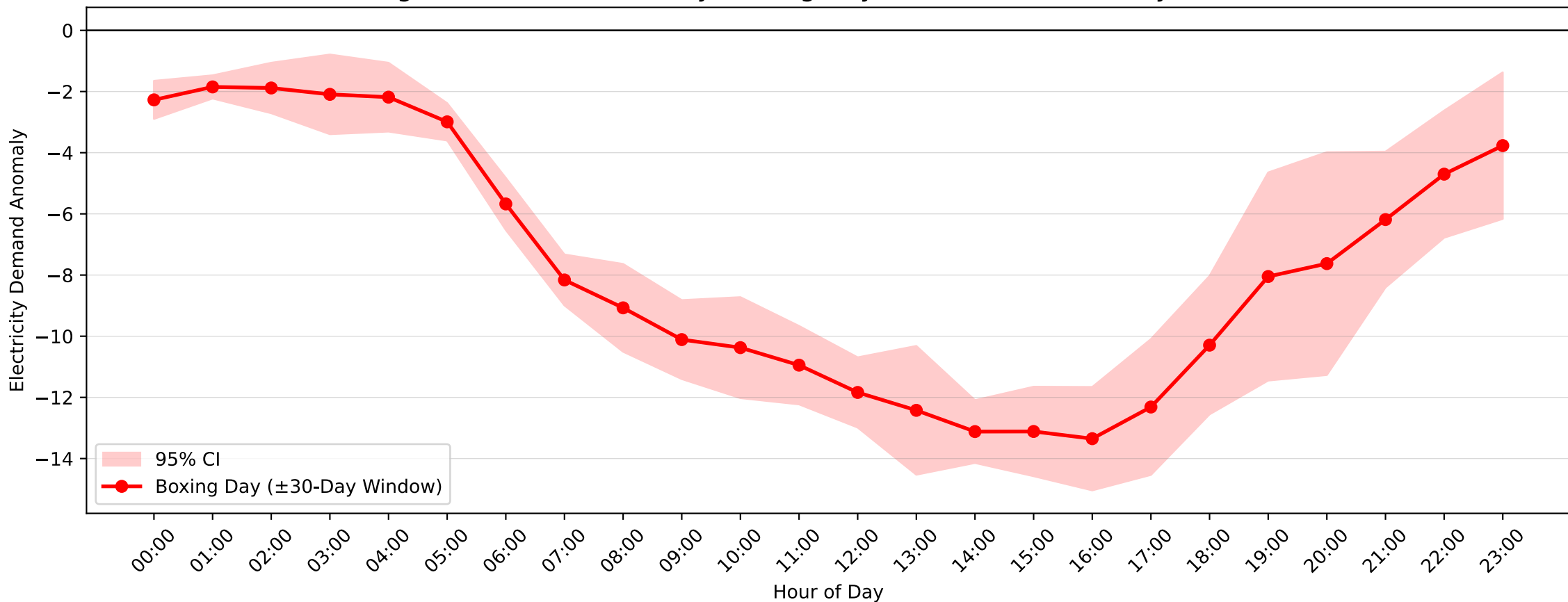
Kogarah Demand Anomaly: Boxing Day (2012-2013, \pm 30 -Day Window)
