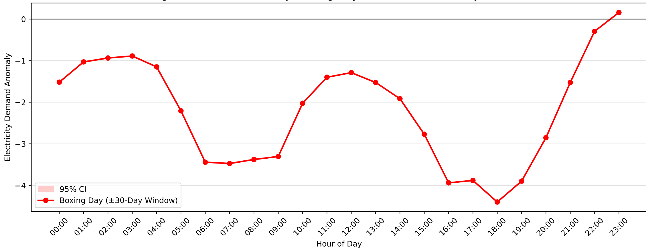
Kogarah Demand Anomaly: Boxing Day (2016–2017, \pm 30 -Day Window)
