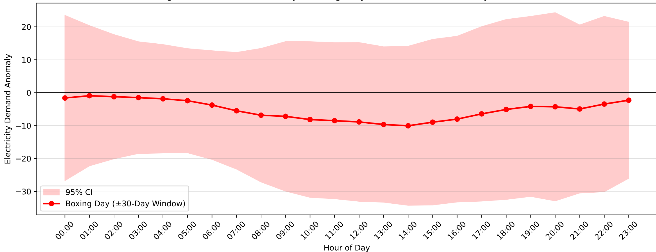
Kogarah Demand Anomaly: Boxing Day (2009–2010, \pm 30 -Day Window)
